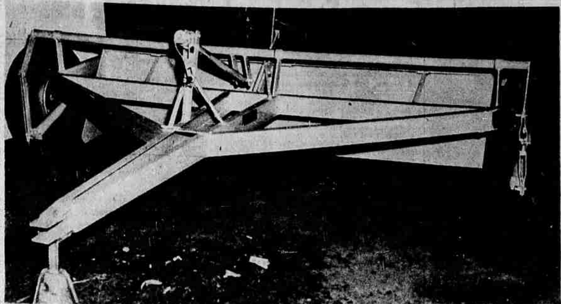
BELIEVED TO BE THE ONLY machine of its kind built on wheels, this checker manufactured by Johnson Machine and Mfg. Co., Malin, is used for building checks for irrigation. A positive depth control with fine adjustment is a feature of the machine.
