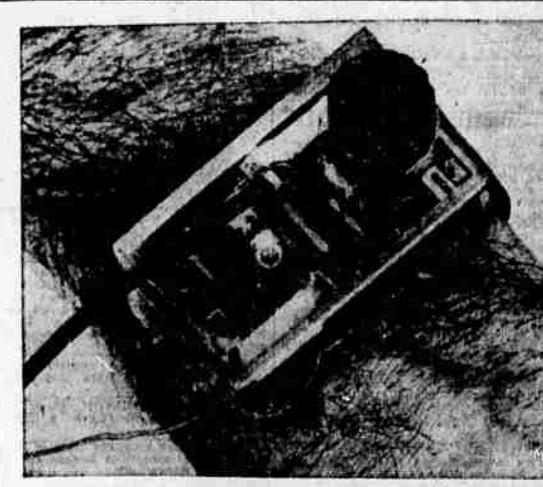
TINY TUNER —Wrist space is usually reserved for a watch, but the Army Signal Corps thinks it's a good place to wear a radio. This is a close-up of the Lilliputian receiver which has transistor-type units replacing the standard vacuum tubes. The knob on the outside of the case is used for tuning in signals. While the unit is unable to transmit, it can pick up signals in a 40-mile radius.
