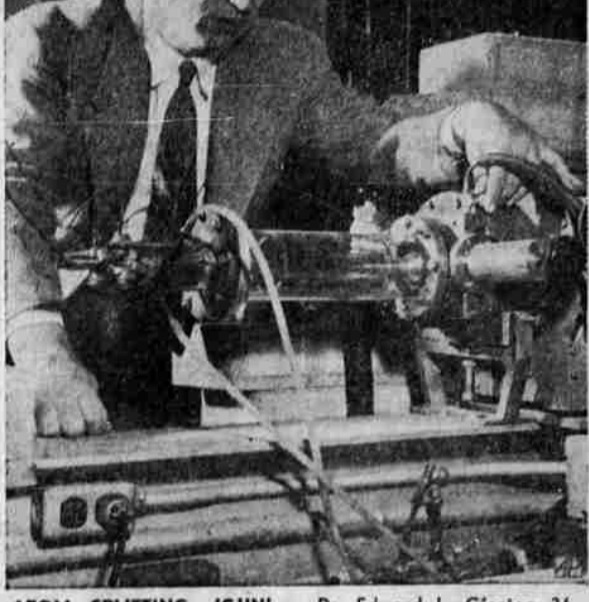
ATOM SPLITTING 'GUN' — Dr. Edward L. Ginzton, 36, (above), director of Stanford University's microwave laboratory at Palo Alto, Calif., adjusts the firing chamber of powerful electron accelerator during a test run of the new atom splitter.
