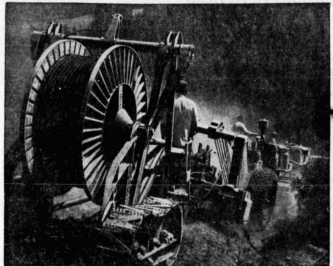
Three machines' work is done by this one... as it digs a trench, lays cable and covers it, all in one operation
