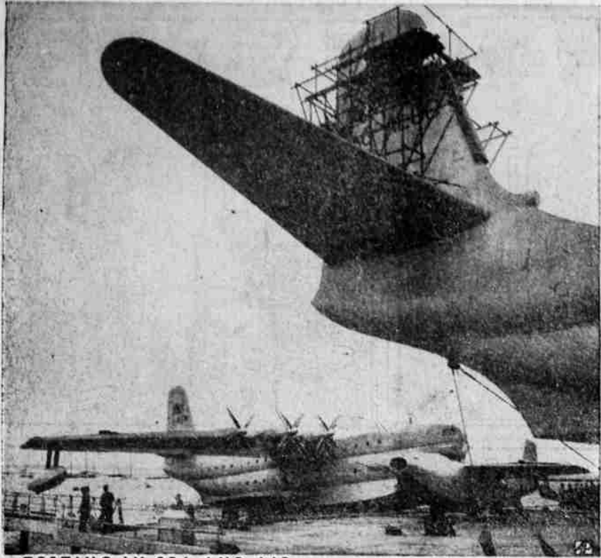
TESTING IN SEA AND AIR —First of three 140-ton "Princess" flying boats, framed by tail of sister ship, slides into sea for taxi and air tests at Isle of Wight, England.
