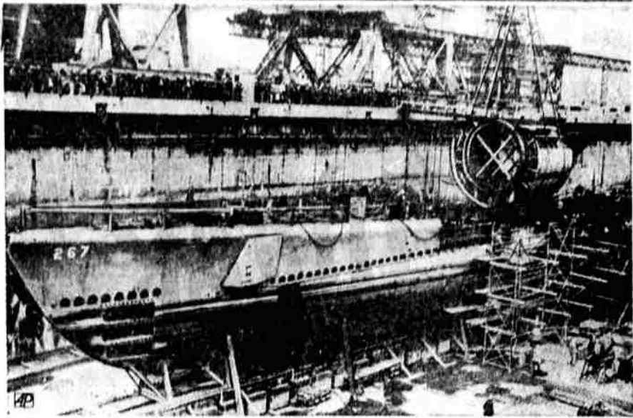
ADDING TO ITS MIGHT—The submarine Pompon lies severed in Philadelphia Navy Yard drydock as workmen lower a new insert with electronic gear into its mid-section.
