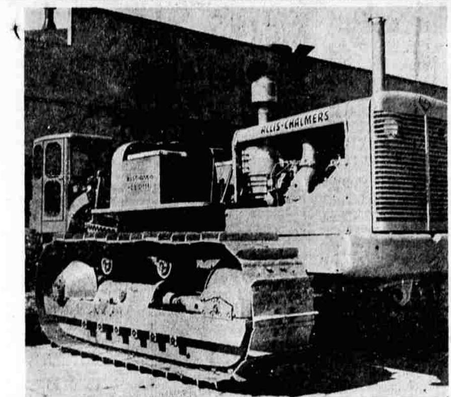
GRAND NEW in the tractor line is this Allis Chalmers HD-9 crawler, on display at West-Hitecock Corp. Weighing more than four tons, this intermediate AC sports 70 horses at the drawbar, 84 at the belt. It has a four cylinder, two cycle GM Diesel engine, six speeds ahead and three in reverse. Unit construction provides easy servicing. The above machine is the first one in this area.
