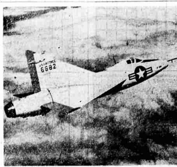
HEADING FOR WILD BLUE YONDER—First photo released of the delta wing Convair XF-92A with afterburner (contained in extended tail section), which adds substantially to the thrust of the plane's J-33-A-29 engine.
