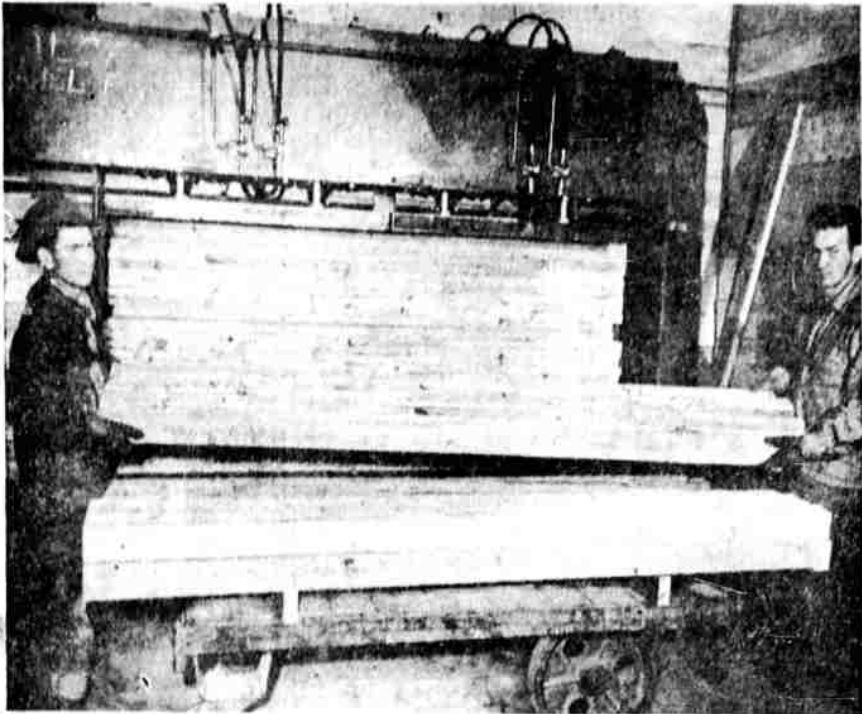
AFTER A HALF-HOUR in hydraulic presses, blocks from the White Pine box factory cutoff saws are no longer waste material. The rough pieces are later planed and dressed for use in construction.
