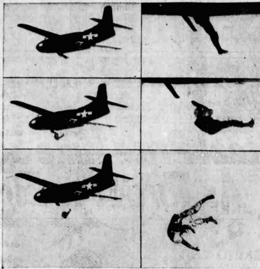
DOWN AND OUT —Unusual photographic sequence above shows demonstration of a new pilot ejection seat being tested on Navy F3D "Skyknight" jet fighters at El Centro, Calif. Conventional ejection device catapults the pilot straight up from his seat. In the F3D the pilot slides down a chute in the cockpit floor and drops out from the belly of the plane. Pictures, starting at upper left and going down, show pilot's course until he is completely free of ship and is ready to pull ripcord of his parachute. Successful "balouts" of this type have been made at speeds up to 430 miles an hour.
