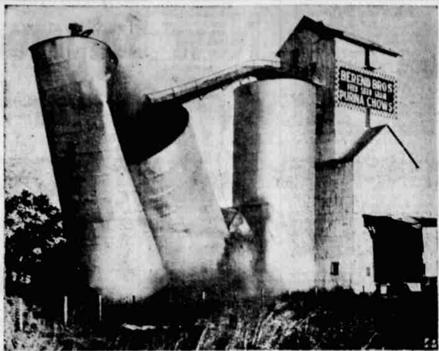
GRAIN ELEVATOR CRASHES —This photo was taken at the instant a 60-foot grain elevator (center) crashed into its neighbor at Wichita Falls, Tex. Grain dust is pouring out the top of the collapsing storage bin while wheat and dust spill out the bottom. A few seconds later, the left elevator, which was empty, also fell. Crash spilled 24,000 bushels of wheat over a 1000-foot-square area. Workmen heard rivets popping, cleared area before crash.
