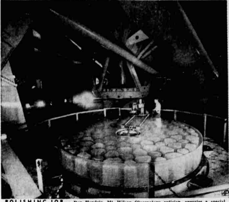
POLISHING JOB — Don Hendrix, Mt. Wilson Observatory optician, operates a special machine to remove 20 millionths of an inch from part of the surface of the 200-inch mirror for the Hale telescope on California's Palomar Mountain.
