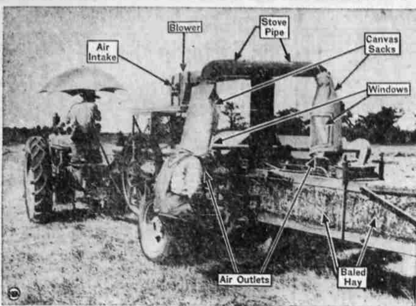
THEY "GET THE SACK" —AND LIKE IT—The men who operate the hay baler on Walter Hahn's farm near Jefferson City, Mo., complained about the heat and dust. So Hahn's son, Herbert, solved the problem with the ingenious air-conditioning device above. The mobile unit consists of a blower operated from the hay baler by a V-belt. The workers put sacks, with transparent plastic windows, over their heads and work in air-cooled comfort.
