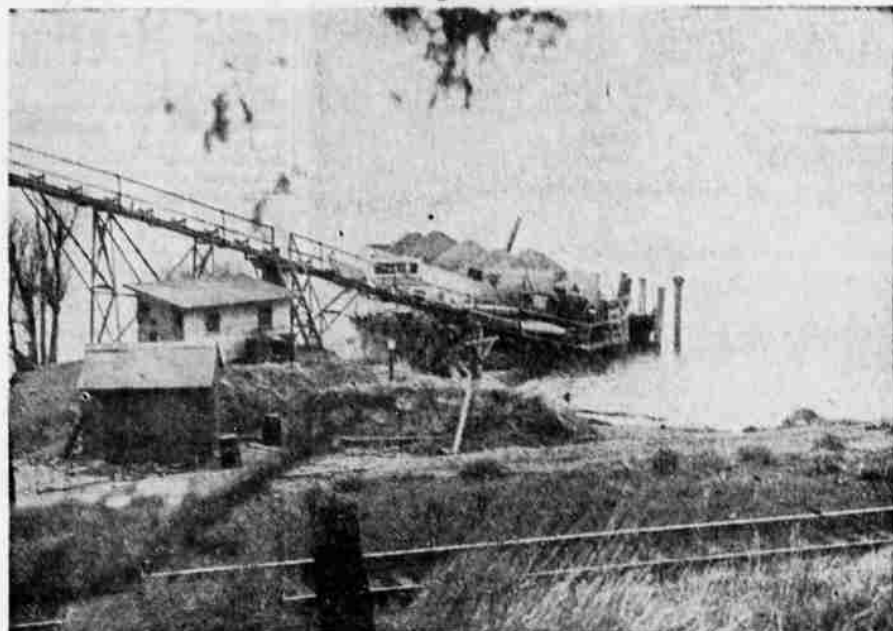
A commercial navigation operation across Upper Klamath lake is conducted by Gladney and Adams, who transport building and ballast materials from pits on the west side of the lake to loading devices on the east side near Modoc Point. This picture shows a steel barge loaded with rock, waiting at the foot of the conveyor belt at the east side dock. Southern Pacific railroad in foreground.
