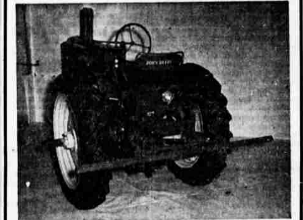
Integral tool carrier with single adjustable tool bar. Takes only 3 to 5 minutes to remove.
