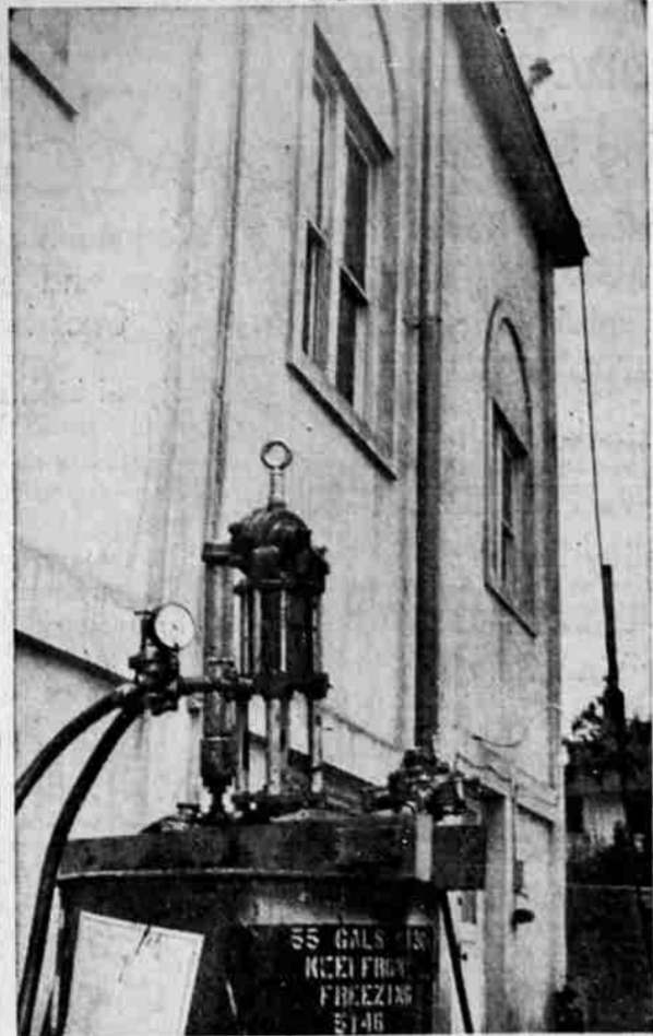
One of the latest developments in construction is this machine which pumps and sprays roofing asphalt. The job was formerly done by hand and is now much speedier and more efficient. The machine is in use by Grem's roofing service.
