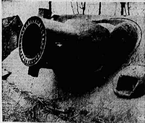
Looks more like something that mixes cement than what it is—a 300-mm. mortar mounted on a modified Mark VI German tank, captured by the U. S. Ninth Army in Oberembert, Germany. The mortar barrel is seven feet long, and fires a five-foot shell weighing 770 pounds. Five-man tank crew was protected by 5-inch armor in front.
