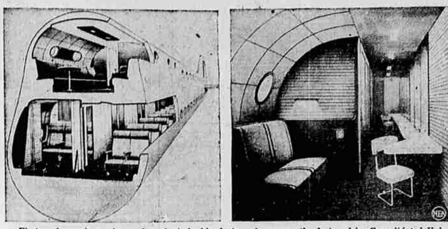
Photos show views of a giant double-decker plane recently designed by Consolidated Vultee, of which 15 are reported to have been ordered by Pan American Airways for postwar passenger service. Twelve times the size of current commercial transports, the super-plane will carry 204 passengers and 15,300 pounds of baggage. A realistic model of the plane appears in top photo. At right, below, is sketch of one of the several compact rest rooms. Cutaway diagram, left, shows passenger space, with luxurious lounge on upper deck, staterooms and comfortable seats on lower.
