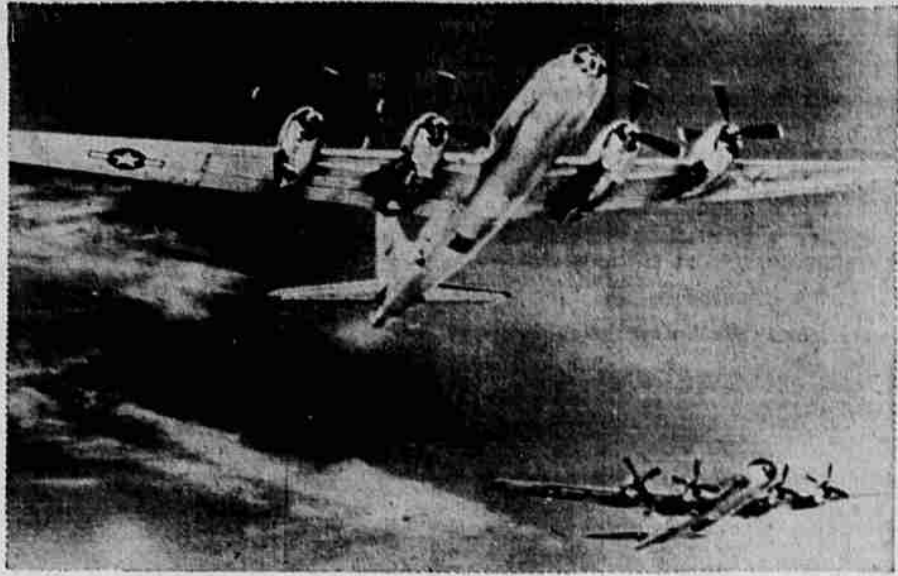
This is the first picture of B-29 Super-Fortresses which attacked Japan proper in what Gen. George C. Marshall hailed as the opening step in new-type offensive against Japanese. Engineered by Boeing and built by Boeing, Bell and Martin aircraft companies, they're powered with four 18-cylinder air-cooled engines of 2200 horsepower each, have speed of over 300 miles per hour and can fly above 30,000 feet. They bristle with guns and cannon, most of which have been deleted from photo for security reasons. U. S. army air force photo.
