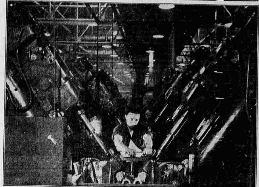
Echoing the valiant "V" chalked up under the very noses of Axis patrols, America's emblematic victory symbol is formed by these machines which angular drill and machine cylinder heads for Pratt & Whitney aircraft engines built by Chevrolet. Three major operations are performed by this battery of machines, whose output contributes to "Volume for Victory," the wartime production principle of Chevrolet.
