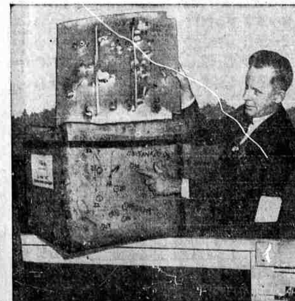
AFTER BULLET BARRAGE—Research Director R. B. Gray examines a new plane fuel tank, tested at Glenn Martin plant in Baltimore. The tank, which is inside a rubber-like casing, was peppered with .30 caliber machine gun bullets. Though the tank wall itself (in right hand) was torn by bullets, the casing had sealed the holes, to prevent fuel leakage.
