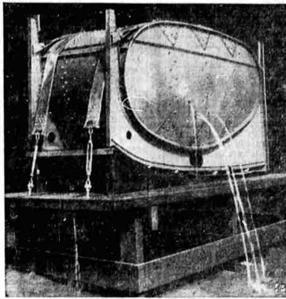
HOW FUEL IS LOST—Water streaming through bullet holes in this old style gasoline tank, pierced by .30 caliber machine gun bullets at a Baltimore test, shows how gasoline might be lost by a plane in flight. The test introduced a new gasoline tank for planes, in which a rubber-like exterior casing "seals up" or "closes over" holes made by the bullets.
