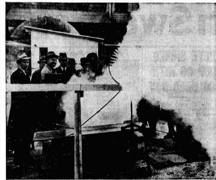
GAS SNUFFS OUT PLANE FIRE —With a great roar a blast of carbon dioxide gas shoots out toward a flaming airplane motor, in a demonstration staged for the Bureau of Standards in Washington, D. C., to show a new C.A.A. device for combating the fire menace in aviation. The gas extinguished the blaze in a 900-horsepower engine within five seconds.
