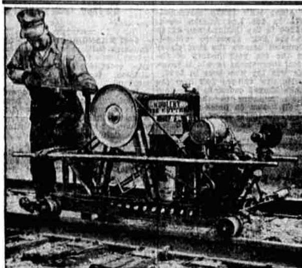
Replacement of railroad ties is not the laborious task it used to be. With motor-driven tie-cutting machines, Great Northern track crews speedily remove old ties. The saw blade, under the operator's left hand, cuts through the tie on the inside of the rail, facilitating easy removal and replacement.
