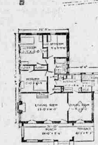
House No. 610 Designed for American Face Brick Association
