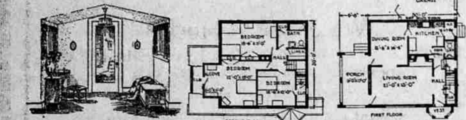
Six-Room House No. 635 Designed for American Face Brick Association
