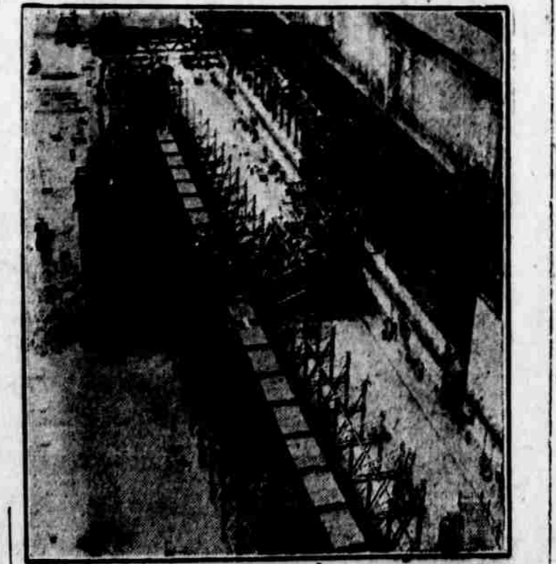
Giant cradle on which the ZR-1, rigid airship, will be built by American engineers at Lakehurst, N. J. The craft will be 675 feet long and 78 1/2 feet in diameter. Small dots at left are human beings, showing vast size of the ship.
