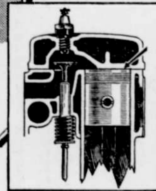
The new high-compression motors have as little as 1/32 of an inch between the top of the piston and the cylinder head—flint carbon is ruinous to them, even in small quantities.
