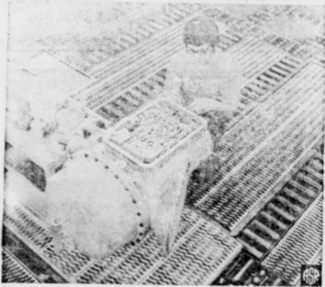
Assorted geometric shapes add an artistic touch to this manufacturing photo taken at Detroit Diesel Allison Division of General Motors in Indianapolis. Featured is one of the firm's new V-730 automatic transmissions for transit coaches. This transmission is the latest technological entry into the burgeoning mass transit industry and represents the first phase of a major expansion effort at the company. Each of the new three-speed automatics goes through a series of static and operational tests by technicians such as Charles L. Acton to verify quality and reliability before shipment to the coach manufacturer. Fluid flowing under pressure through the intricately carved channels of the valve body (in front of Acton) activates a series of valves. These in turn control the automatic-shifting components. Completing the picture are the roller conveyors and perforated walkways covering the production floor.
