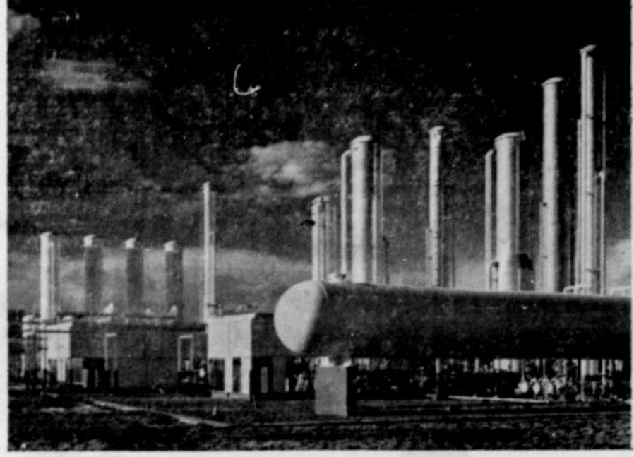
PROCESSING TOWERS are designed to remove gasoline from product of Natural Gas wells. Other by-products are also removed in purification process, leaving only pure, clean heat energy for a variety of uses.
