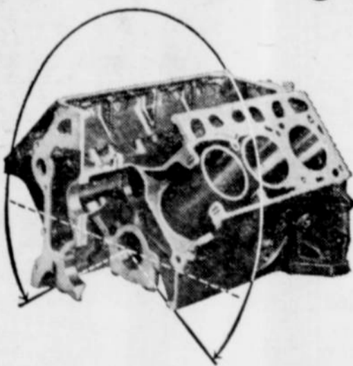
New Ford Deep-Block design gives highest structural rigidity of any truck engine! Main bearings get full 240° support. Smoother high-compression performance! Longer life! More efficient operation! Proven in a billion miles of trucking!
