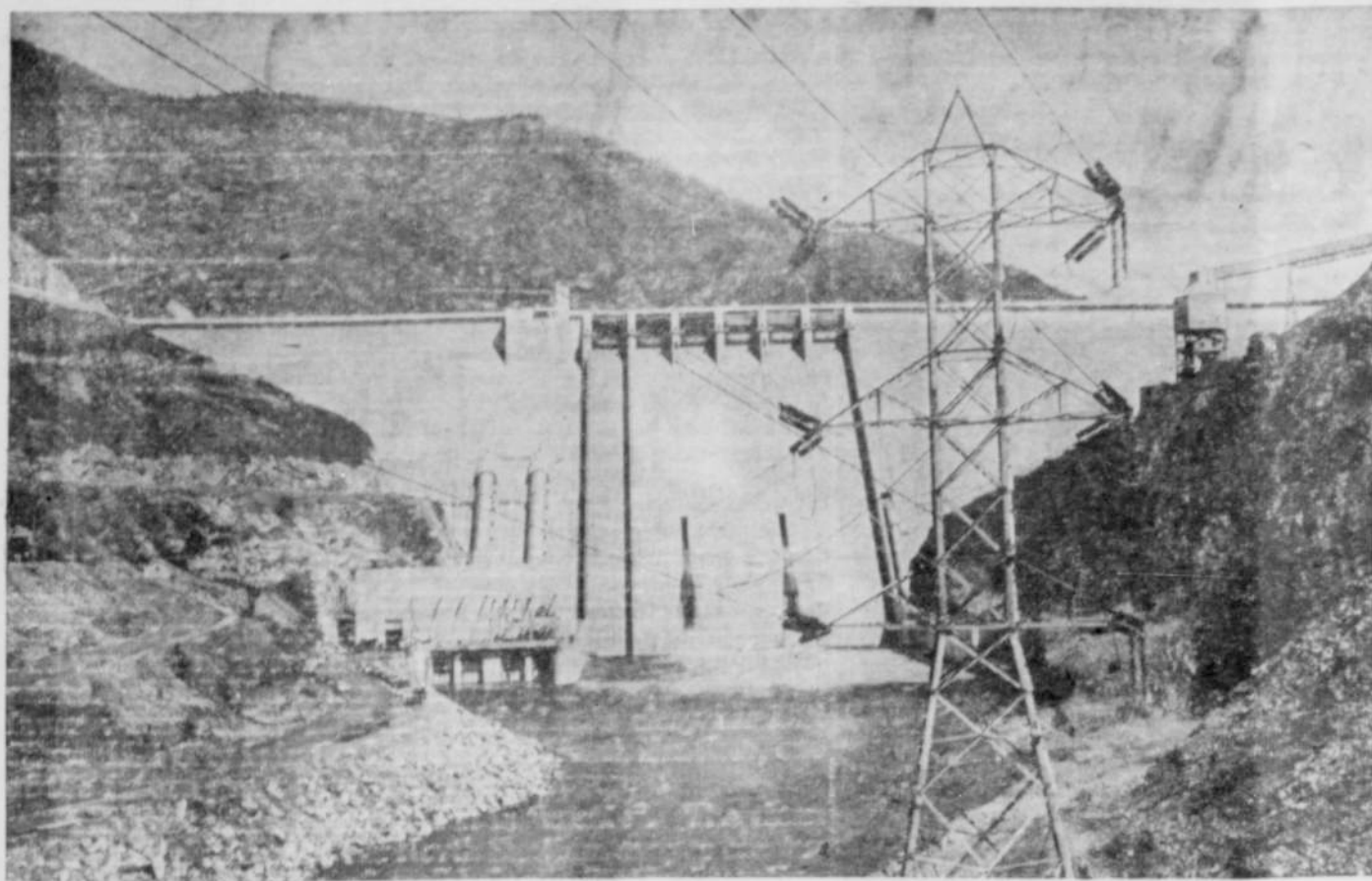
Multi-purpose Detroit dam designed for flood control and generation of 100,000 kilowatts of power, constructed at a cost of $70,000,000, was dedicated June 10. This concrete, gravity type dam has a total length of 1580 feet and a maximum height from foundation to deck of 154 feet. Impounded behind the structure is Detroit dam reservoir eight and one-half miles in length and holding approximately one and a half billion gallons of water amounting to a storage of 455,000 acre feet. (Photo courtesy Capital Journal)
