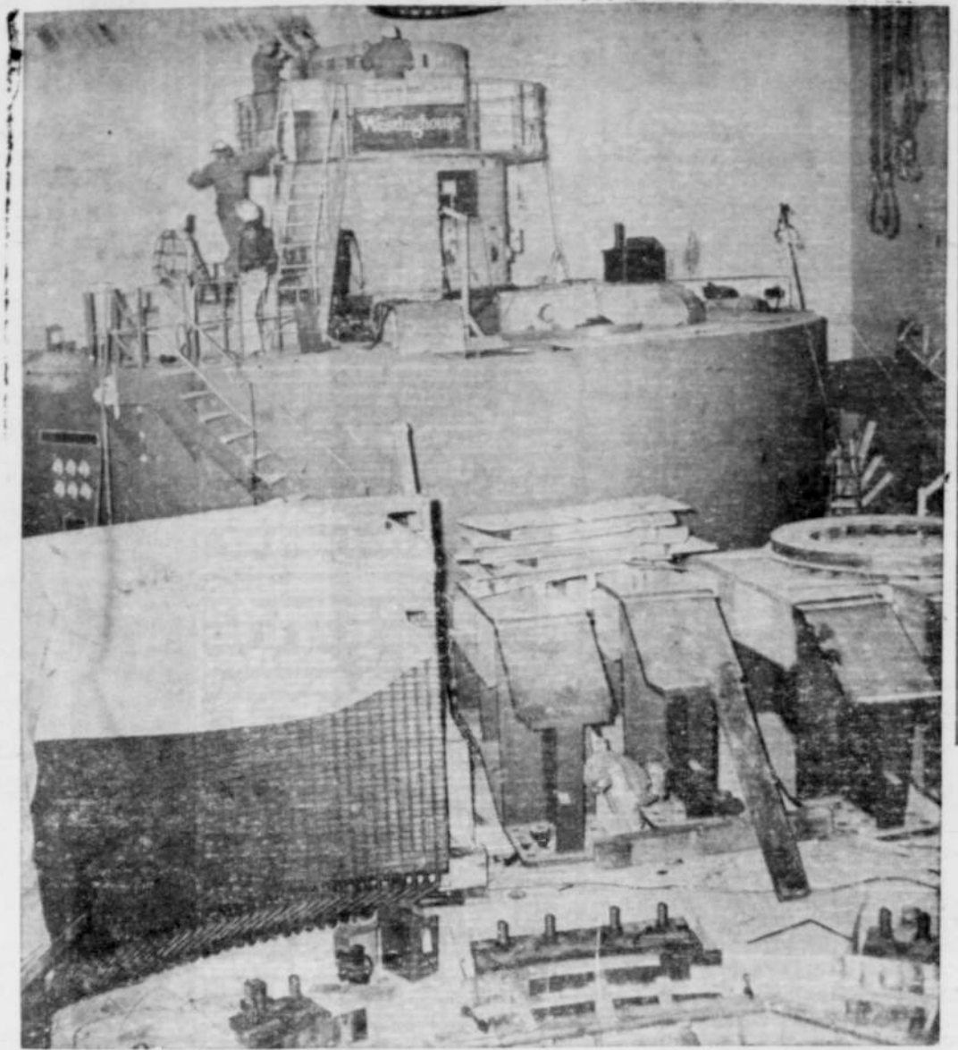
Multi-purpose Detroit dam designed for flood control and generation of 100,000 kilowatts of power, constructed at a cost of $70,000,000, was dedicated June 10. This concrete, gravity type dam has a total length of 1580 feet and a maximum height from foundation to deck of 154 feet. Impounded behind the structure is Detroit dam reservoir eight and one-half miles in length and holding approximately one and a half billion gallons of water amounting to a storage of 455,000 acre feet. (Photo courtesy Capital Journal)
