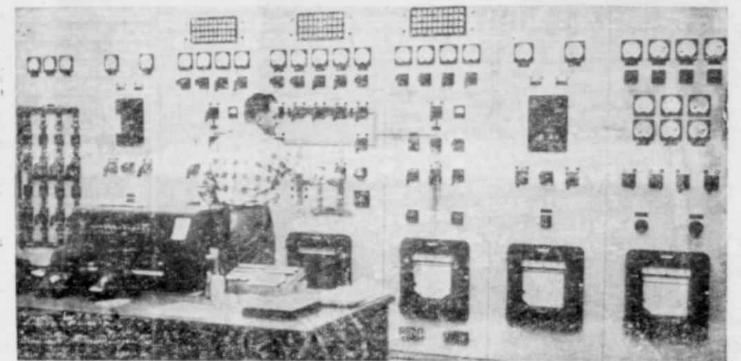
One of two 50,000 kilowatt generators in Detroit Dam powerhouse was found to have lost a bearing the day before the scheduled pressing of a button on June 10, and will be delayed for several weeks. Powerhouse generators are turbine fed by penstocks 15 feet in diameter. Combined output of Detroit's generators will be 100,000 kilowatts of power. Lower: Control panel for the three generators associated with Detroit dam shown with B. E. Whitsett, Jr., senior operator for the corps of engineers, at one of the controls. (Photos courtesy Capital Journal)
