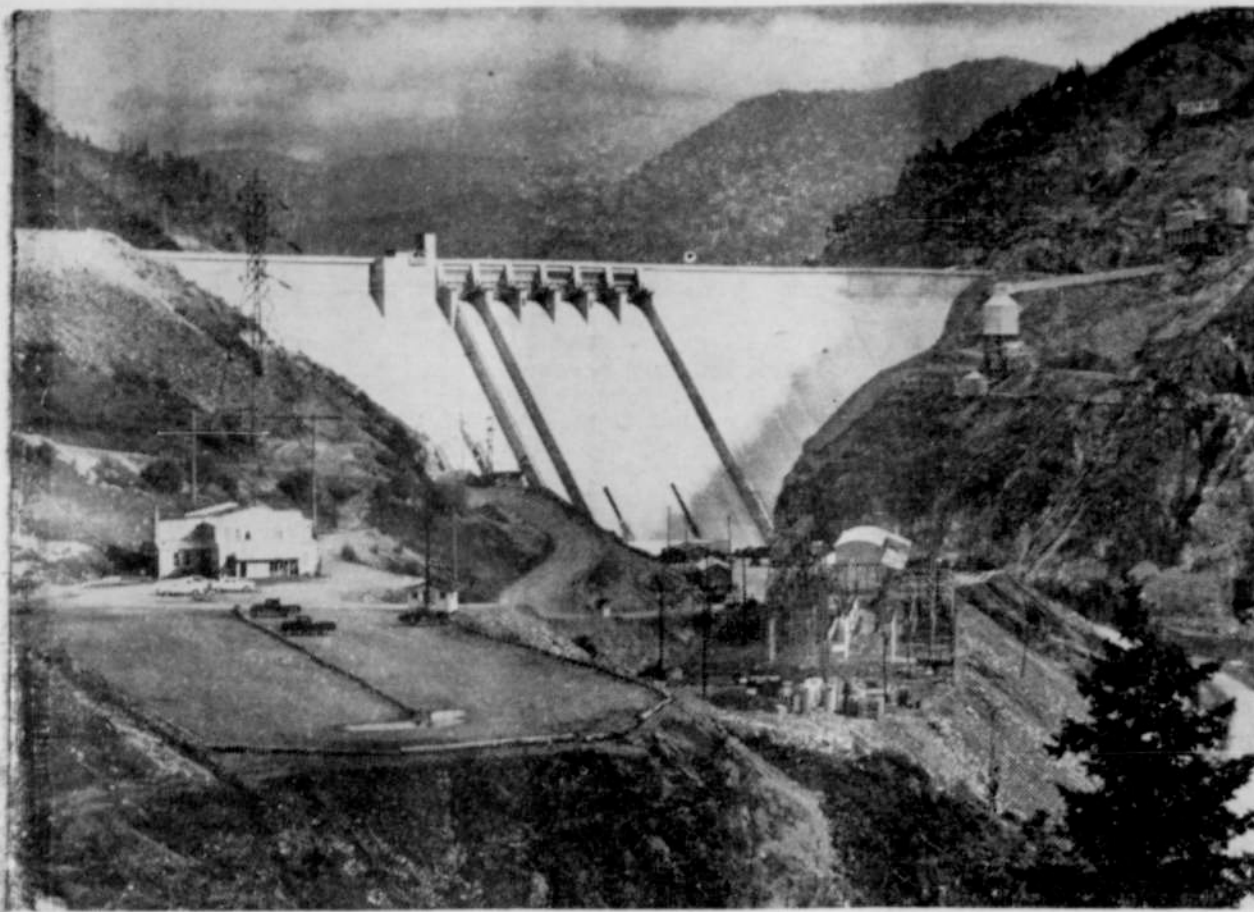
Majestic Detroit Dam shimmers in afternoon sunlight as final preparations are made for its dedication today. The event is the high point in seven years of construction activity on the project, but work will continue on smaller scale for another year. Powerhouse and Big Cliff Dam remain to be finished. Building in left foreground is headquarters of Consolidated Builders, Inc., contractors. (Photo courtesy The Statesman)
