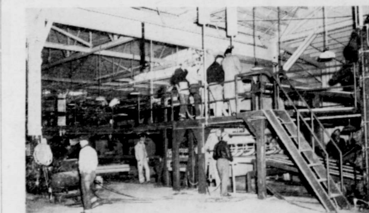
Workers in new veneer plant of the M and M Woodworking Co., at Lyons, operate cutting and sorting machine as huge mill began operations Monday. The plant operates as a straight production line. Starting at west end of mill, logs are cut to standard length, barked, then the veneer is cut in a huge lathe and the strips carried on endless belts to the cutting machine where it is cut into commercial sizes, graded and packaged for delivery. (Photo courtesy The Capital Journal)
