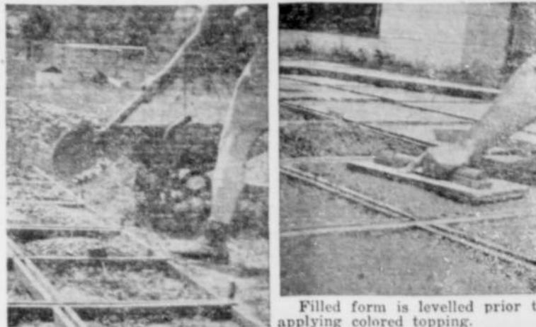
Greased form, set on levelled ground, is filled with concrete.
