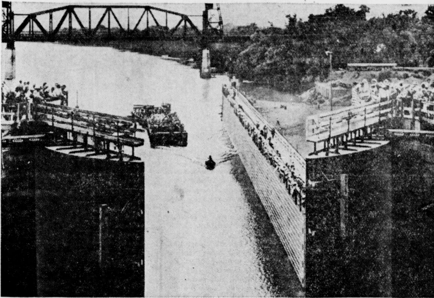
Citizens of Chattanooga, and surrounding area recently witnessed the initial opening of the navigation lock of Chickamauga dam by the Tennessee Valley Authority. The dam is now under construction. At normal level the lake that will be impounded by the dam will cover approximately 32,000 acres. It is located about seven miles from Chattanooga. The actual opening of the lock is pictured here.
