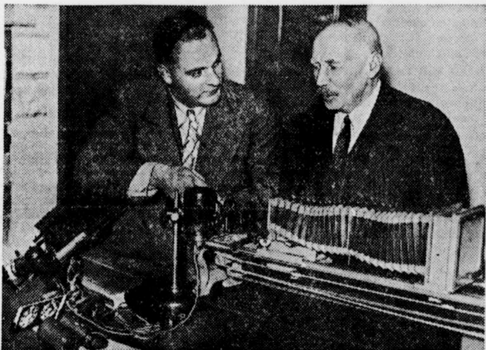
William B. Spooner (left) and Frank F. Heitzler, both of Boston, the inventors of a new third dimension diamond camera by the use of which photographs can be made through a diamond to show all defects and cuts so that a stolen stone can be identified in a matter of minutes by police departments, are shown. Without their camera it is impossible to make a positive identification of a stone after it has been in use for any time. The diamond is recorded in much the same way that finger prints are recorded.
