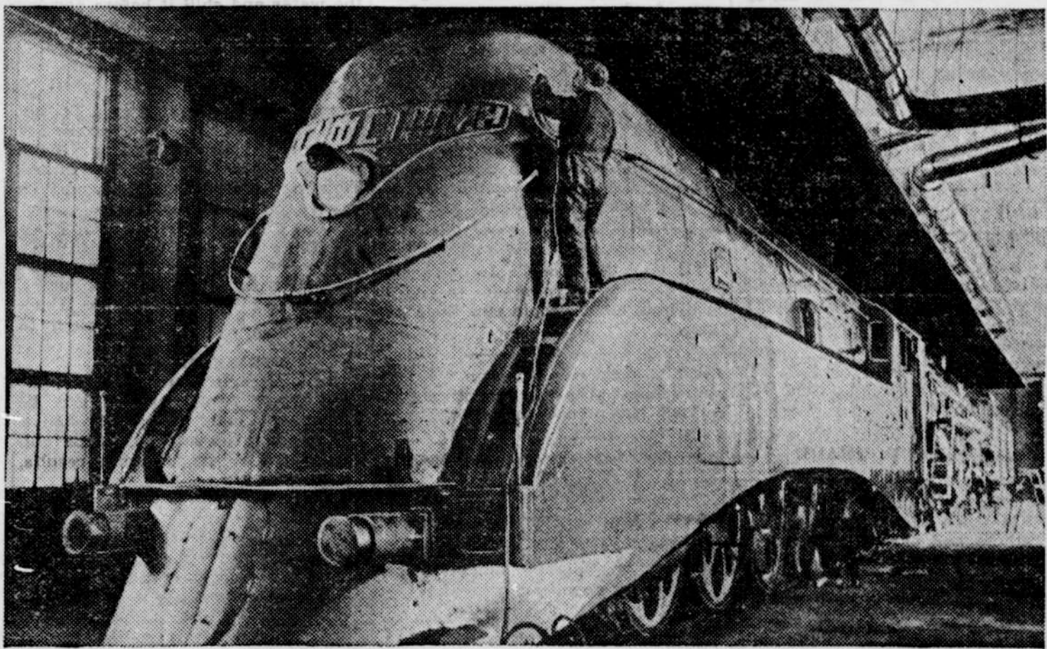
Following the lead of American railroads, the Russians are now streamlining their locomotives. The "Joseph Stalin," built at a government locomotive works in the Ukraine, is pictured ready for a trial run. It is designed to run at a speed of 85 miles an hour.
