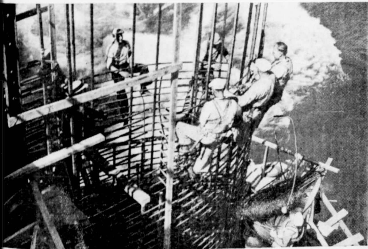
Clouds just over their heads and white caps below their feet are all part of the job to the workers who are building the steel reinforced structure for mighty Bonneville Dam on the Columbia river. This power navigation flood control project financed by the Public Works Administration at a cost of $32,000,000 is being undertaken under the direction of the Army Corps of Engineers.
