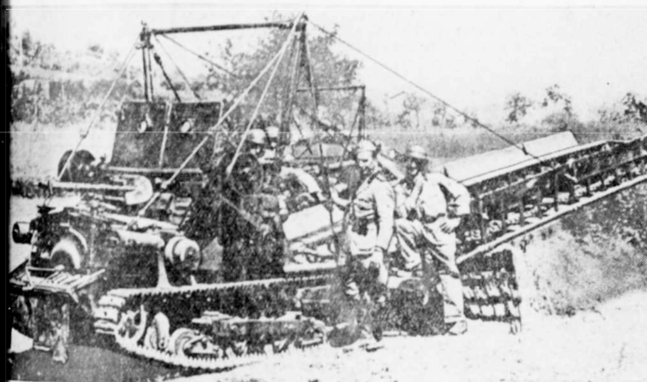
This is a new Italian tank which carries a bridge for transporting soldiers over small rivers. It was demonstrated for the first time at the huge Italian war maneuvers held near Avellino recently.
