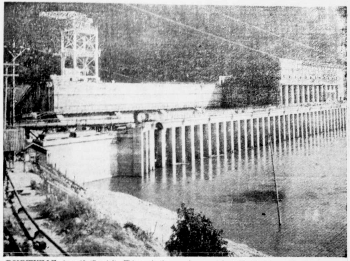
BONNEVILLE, Aug. 12 (Special) —This project's powerhouse—at least the first two units of it—wears an almost completed aspect, with pouring of roof concrete all but ended and interior installations proceeding rapidly. The Columbia, now flowing a mere 150,000 cubic feet per second, is much more placid than it was three months ago, when the flow was more than triple the present figure.
