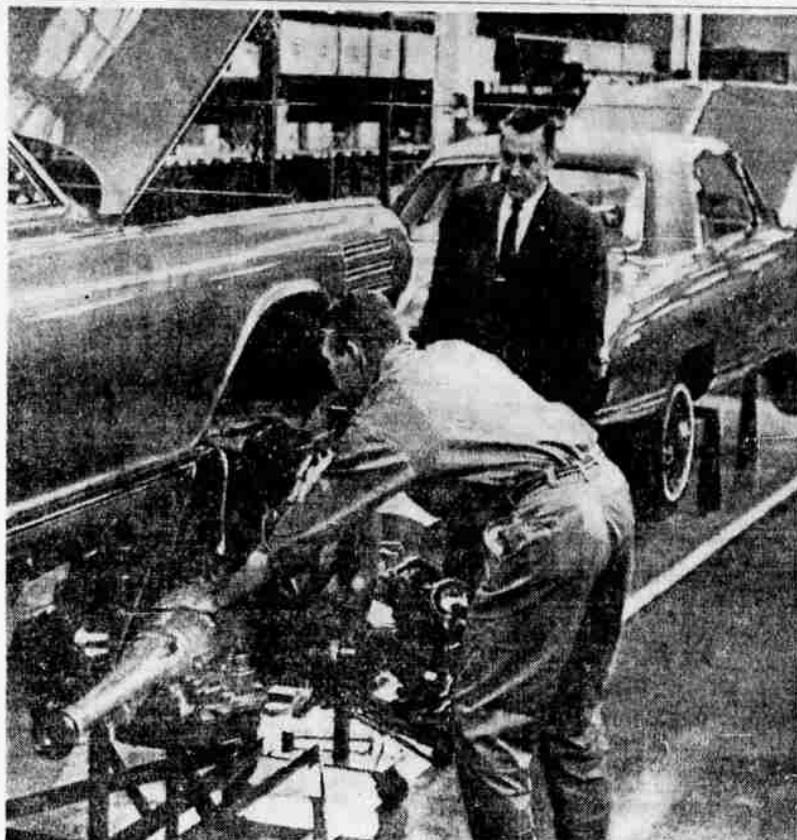
ENGINE INSTALLED — Chrysler President Lynn A. Townsend watches as technicians install a new turbine engine on what is the world's first assembly line for gas-turbine passenger cars. The engine, mounted on the front suspension system, is being fitted to one of the first 50 consumer test cars. (UPI)
