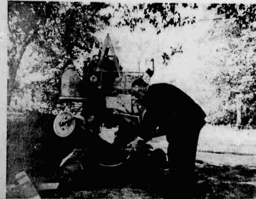
The wrapping machine, being inspected by Mr. Hoppe, is a new and unusual machine in this industry, using polyethylene wrap. In one revolution it covers two feet of pipe.
