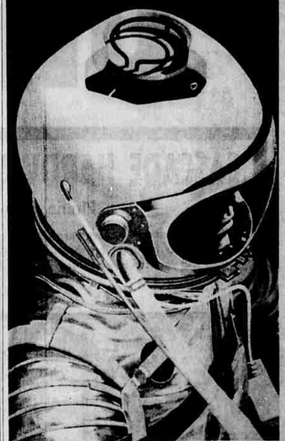
ANTENNA IN HAT —This cutaway sketch shows a tiny ring-shaped radio antenna in an astronaut's helmet to provide communications to earth from an orbiting spacecraft without use of a projecting whip antenna. It also eliminates need for a connecting cable to the space vehicle's communication system, and is applicable for use by jet plane crewmen and paratroops. It is designed by Northrup Ventura at Newbury Park, Calif. (UPI)
