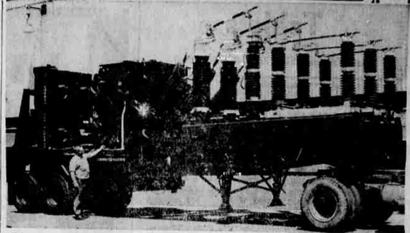
TROUBLE-SHOOTER —Looking more like a science-fiction artist's conception of an atomic dreadnaught, this work-a-day piece of equipment is a mobile substation now stationed in the Copco division of Pacific Power & Light company's system in southern Oregon and northern California. It can be ready to roll within minutes to take over power substation function when regular facilities are out of service due to emergencies or for regular maintenance work.
