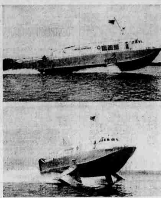
ON OWN FOILS -The experimental hydrofoil Denison starts to lift off the water, top, and flies away on her foils. The strange looking craft is undergoing a series of tests off Newport, R.I. Powered by a 14,000 horsepower jet turbine engine, she is capable of making 60 knots. (UPI)
