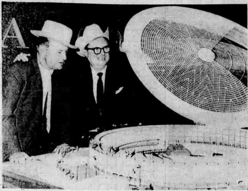
WORLD'S FIRST—Model of world's first domed, air-conditioned, all weather, all purpose sports stadium... to be completed in Houston, Tex., in late 1964 for use by Houston Colt .45's and American Football League
