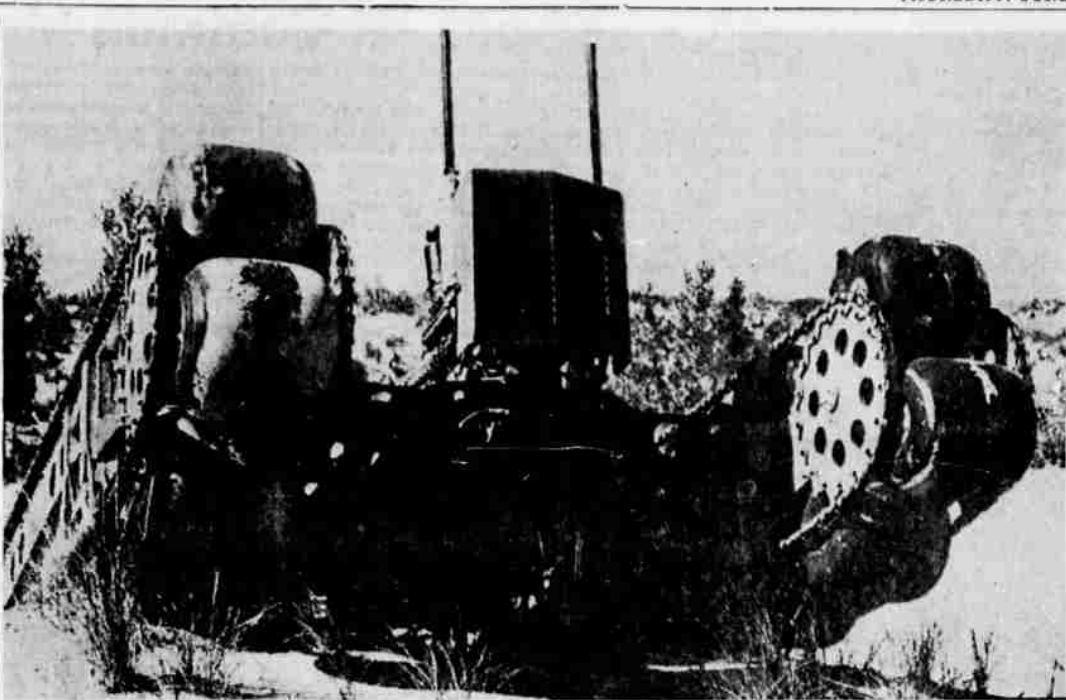
NEW CONCEPT IN TRANSPORT —This new Navy vehicle is known as the Airoll, a new concept in off-the-road transport. The free-rolling tires mounted on the endless chain can take the 19,000-pound vehicle over ordinarily impossible terrain, such as deep mud, heavy snow and watery swampland. It has 16 tires on each track. (UPI)
