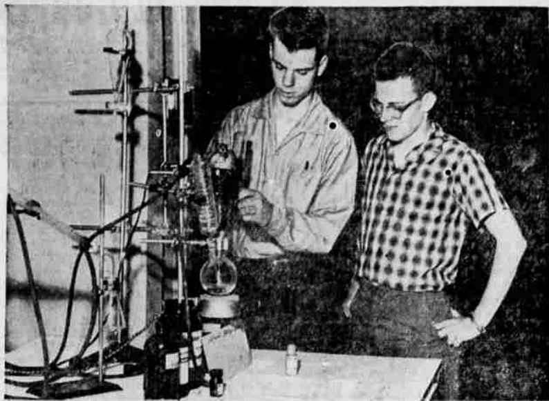
ORGANIC SYNTHESIS —Illustrating chemistry instruction offered at Medford High school is this exhibit by Mark Hadley, left. Looking on is Jim Moyer. Hadley is using a grignard reaction apparatus. It is used for organic synthesis. Work in various departments of the high school was on display for Rotary and Kiwanis club members last week at Rogue Valley Country club. Moyer had a display of actual naiads and artificial naiads he had made.
