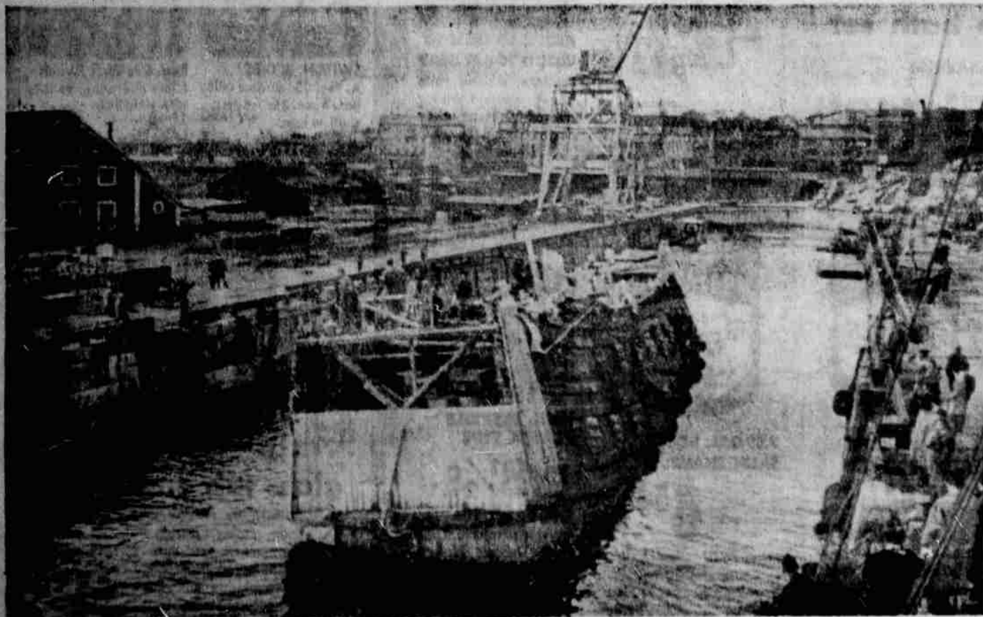
FLAGSHIP LIFTED —The Wasa, flagship of King Gustavus Adolphus' fleet, lists only slightly in Stockholm after having been lifted from the bottom of the harbor where it had rested for 333 years. The ancient Swedish warship capsized and sank on its maiden voyage in 1628 with 500 aboard. It is being prepared for conservation as a floating museum. (UPI Telephoto)
