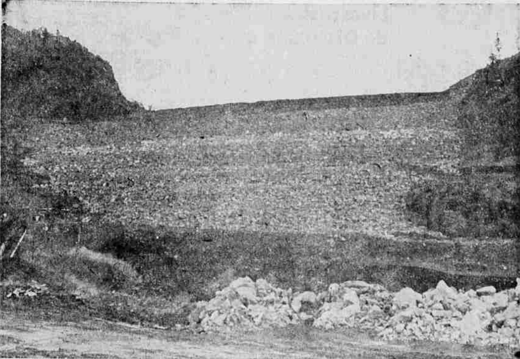
OUTER FACE — The outer face of the dam, shown above, faces approximately north. Although it looks steep because of foreshortening in the photo, it actually has a fairly gradual slope, as shown in diagram elsewhere on this page.
