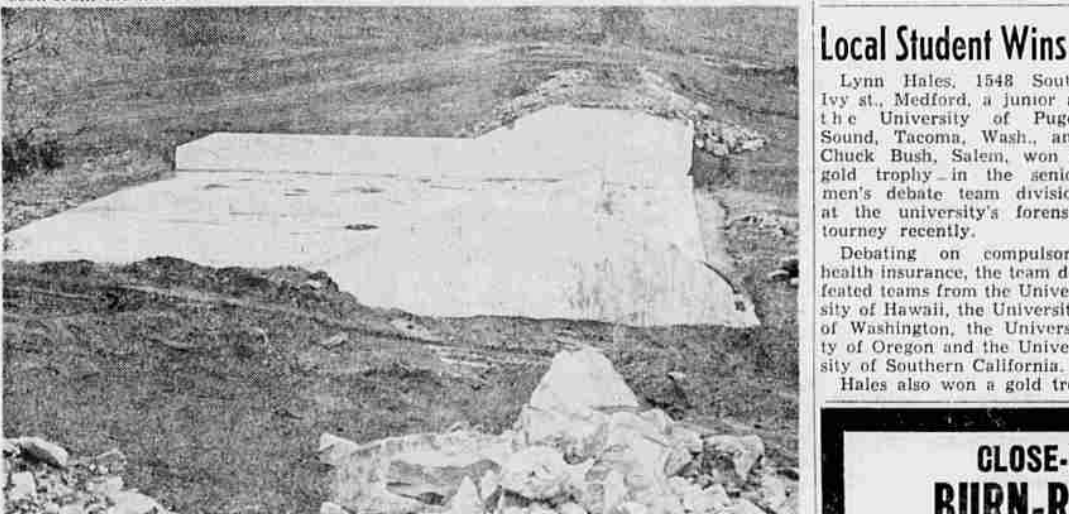
GENERAL VIEW — A general view of Emigrant dam, seen from the hill southwest of the structure and south of the west abutment, is shown above. The water level here is somewhat higher than the maximum pool with the old dam.
