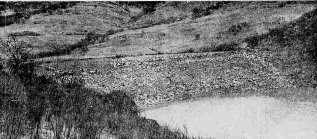
HIGHWAY SADDLE DIKE — The dike shown above is in the saddle through which the Green Springs highway used to run before it was relocated (a portion is visible at right of dike), and is near the spot on the lake formerly most used for recreational purposes. Though smaller, it is of a type of construction identical to that used in Emigrant dam.
